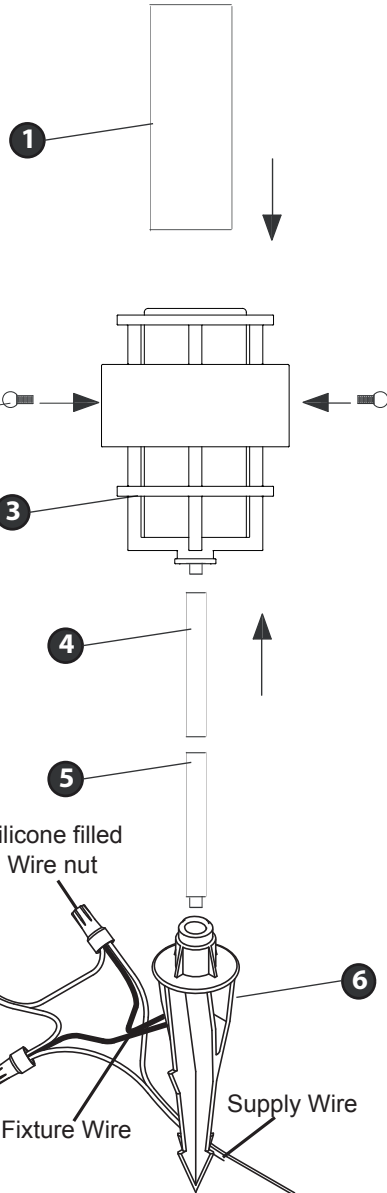
DRAWING 1 - Fixture Installation
