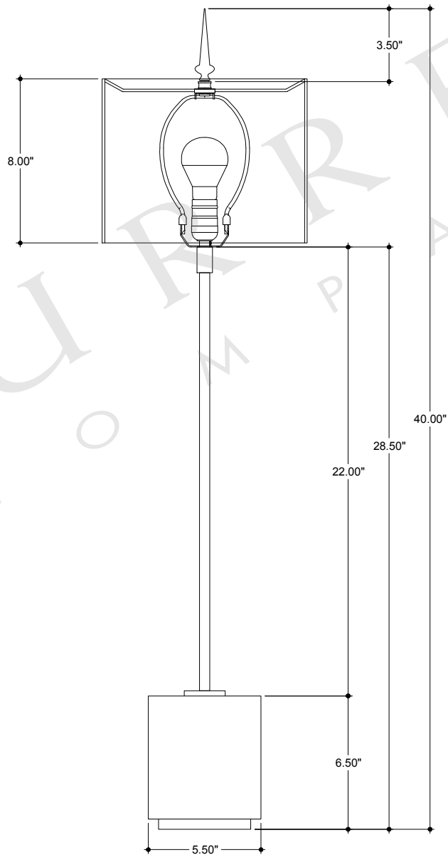
FRONT VIEW
