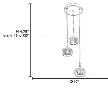
LINE DRAWING
