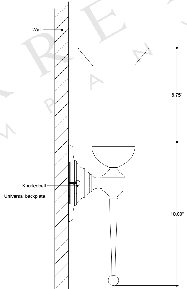
SIDE VIEW
