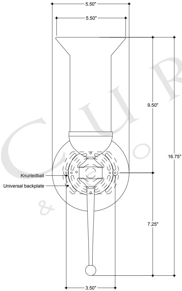
FRONT VIEW
