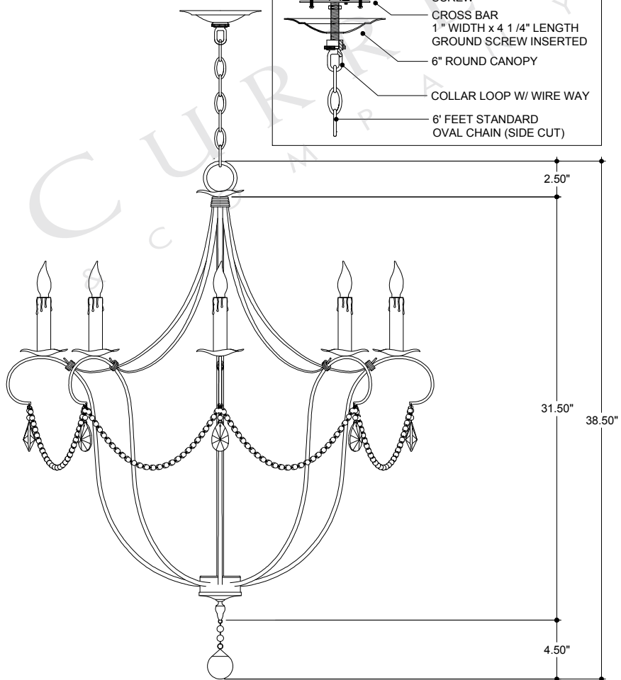
FRONT VIEW
