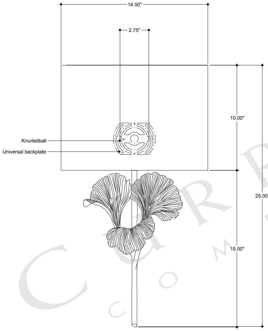
FRONT VIEW
