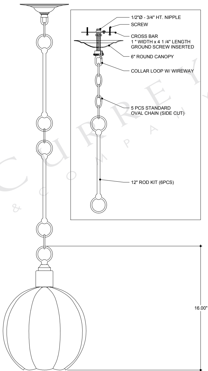
FRONT VIEW
