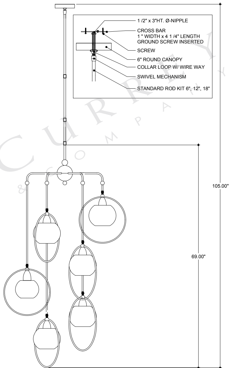
FRONT VIEW
