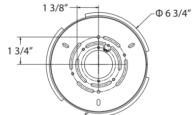
Back Plate Dimensions
